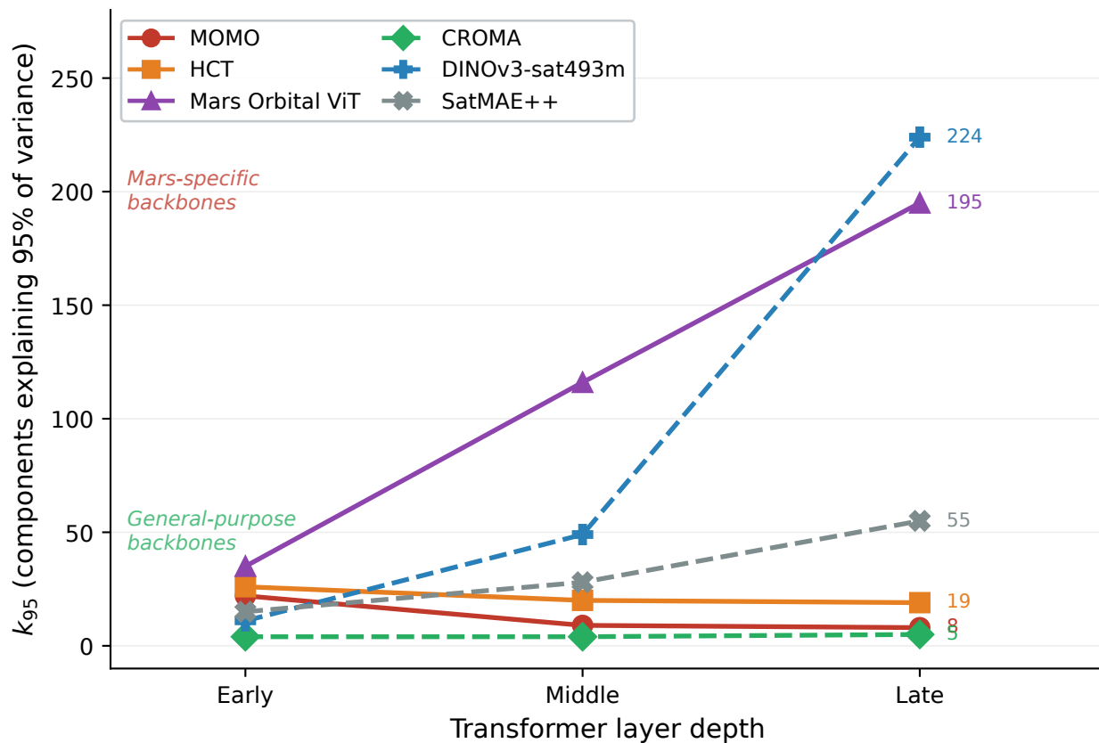
Effective dimensionality across backbone and depth
